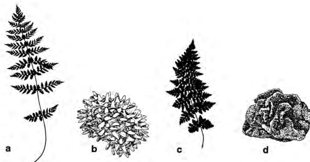
Leaf shape and spores morphology of Cystopteris : (a, b) C. fragilis , (c, d) C. dickieana .
